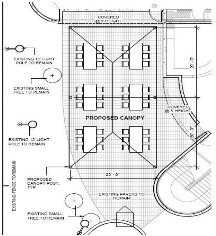
Proposed site plan for new awning on west side of building
